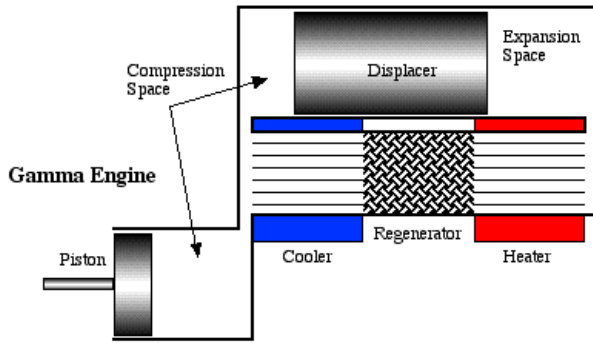
Figure 3.1. c) A typical gamma-type engine.
