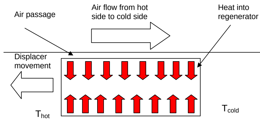
Figure 2.7.1. a) Heat transfer occurring from the hot air to the regenerator as the air moves towards the cold space.
