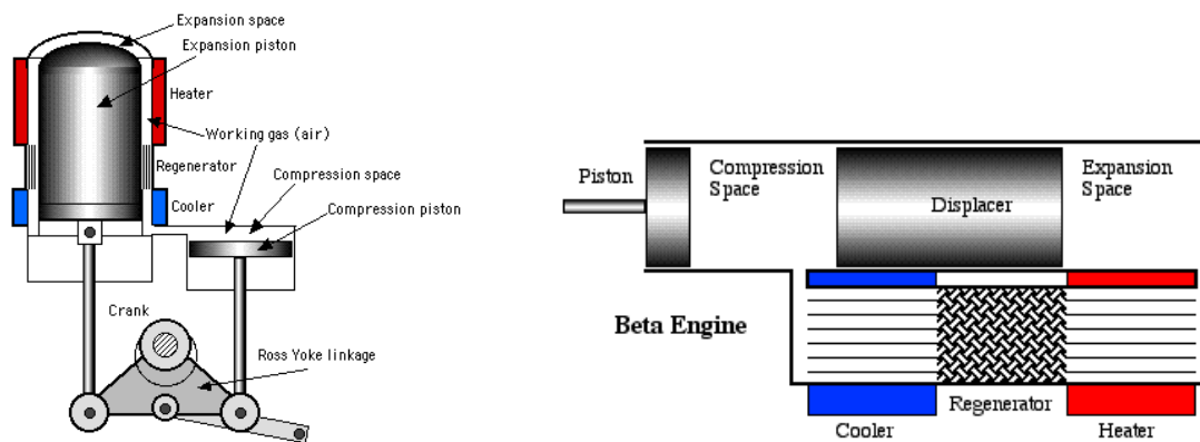
Figure 3.1.a) A typical alpha-type Stirling engine. b) A typical beta-type Stirling engine.
