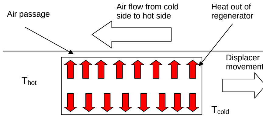
Figure 2.7.2. b) Heat transfer from the regenerator to the working gas as the cold air moves towards the hot space.
