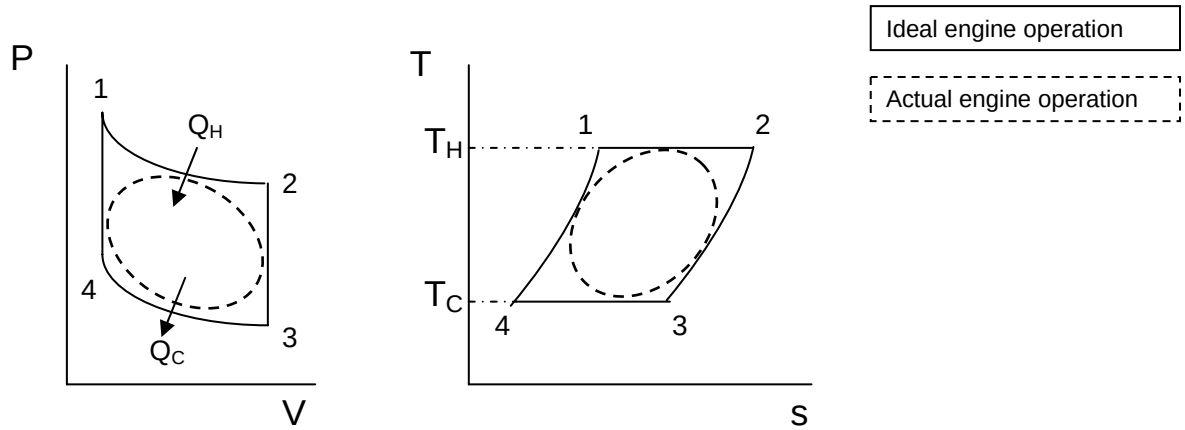
Figure 1.4.1: Stirling cycle Pressure-Volume and Temperature-Entropy diagrams
