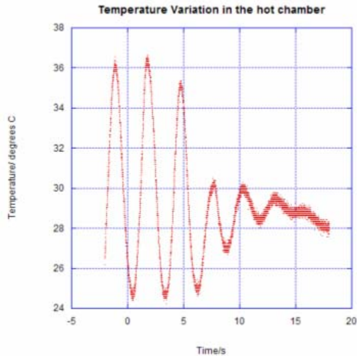
Figure 5.1.2 Graph of temperature variations inside hot cylinder; max temperature during free-oscillation was observed to be 30°C.
