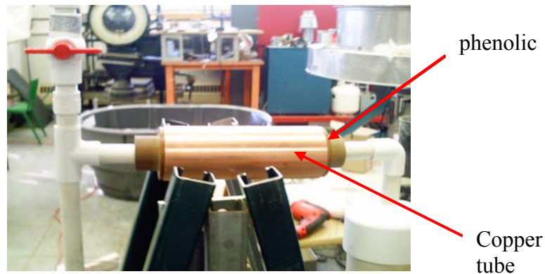
Fig 4.2.1: Picture of the heat exchanger
