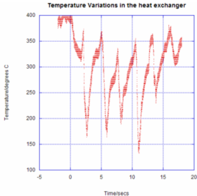
Figure 5.2.3 Heat exchanger temperatures varied between 125°C and 400°C.
