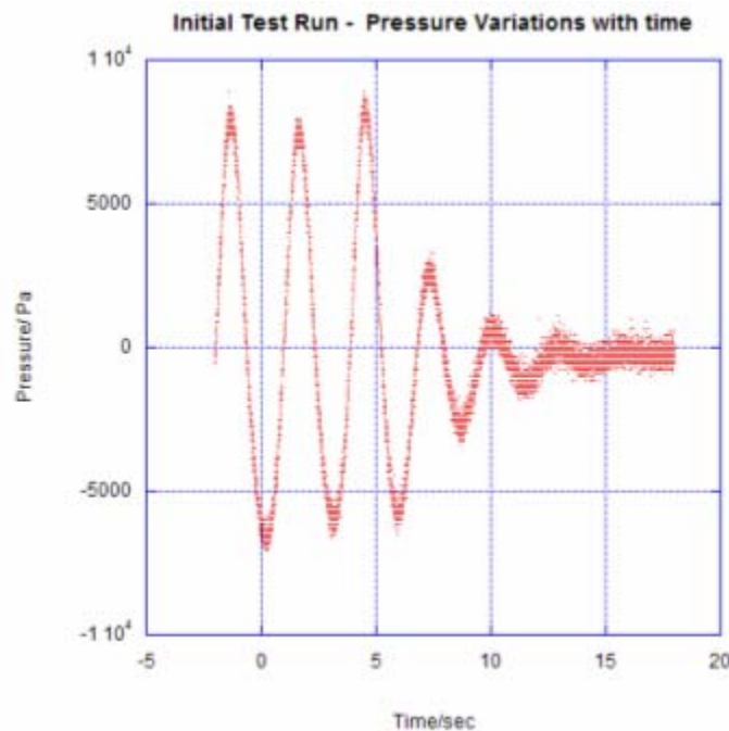
Figure 5.1.1 Using heat device from hair dryer the maximum pressure recorded was 8kPa and the maximum pressure during free oscillation was 2.5kPa; the decay time constant was 5 seconds.
