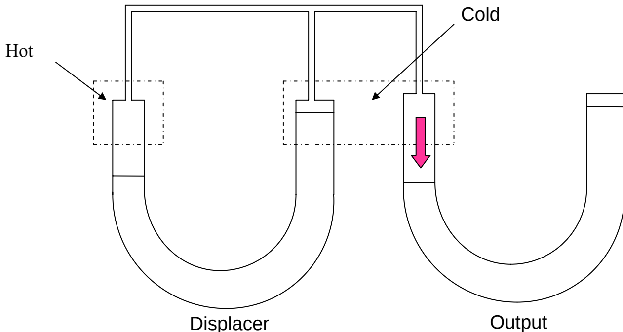
Fig 1.5.1: Basic schematic of a fluidyne
