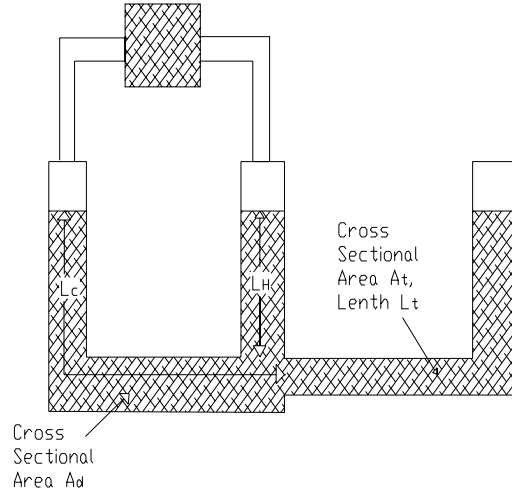
Fig 2.4.1: Tuning column configuration with merged cylinders
