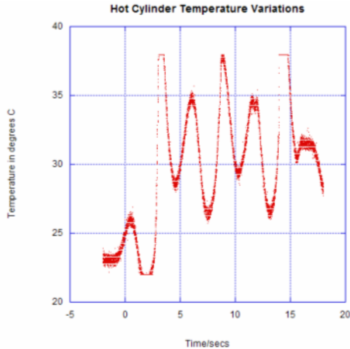
Figure 5.2.4 Temperature varied between 23°C and 37°C in the hot cylinder.
