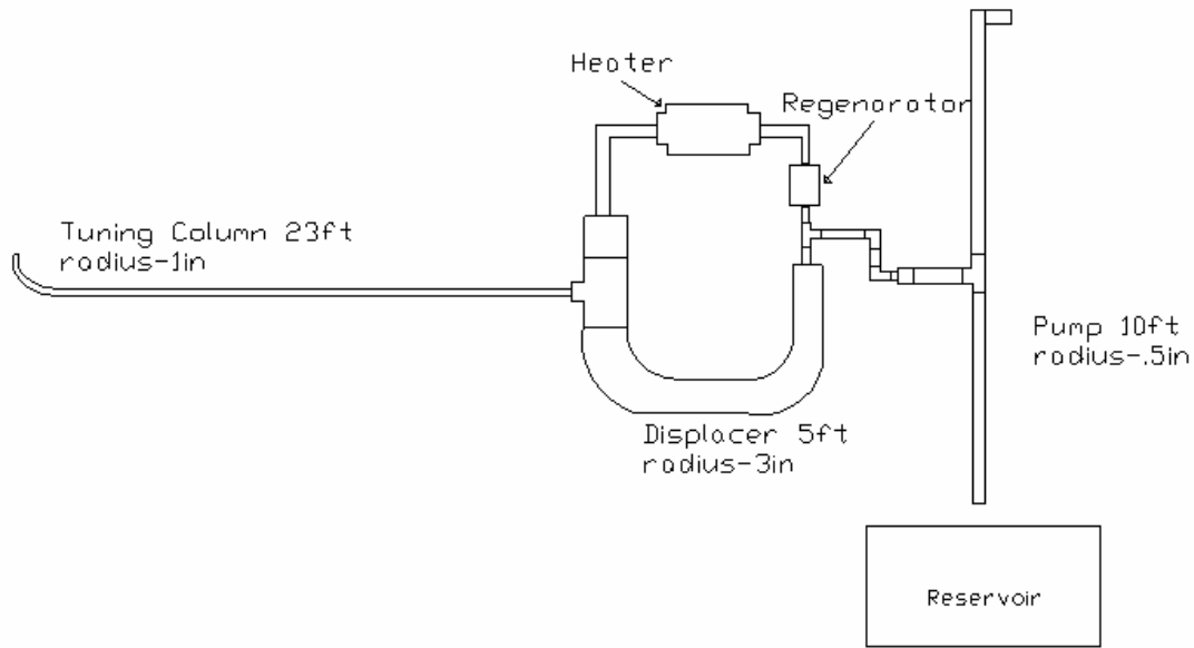
Fig 3.1.1: Design diagram of our fluidyne pump
