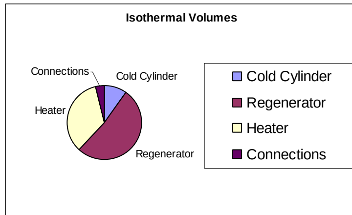
Fig 3.1.2: Isothermal Volumes
