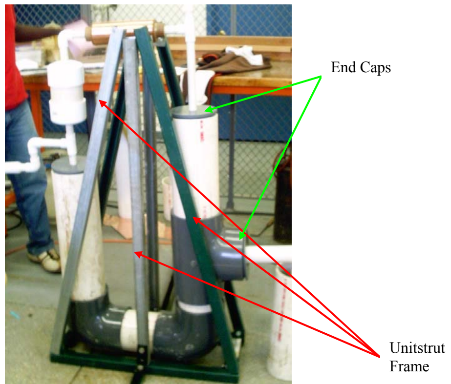
Fig. 4.2.2: Picture with Unistrut frame
